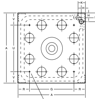
(4) MOUNTING HOLES 3/8" - 16 FOR MODELS 104-367 THREAD TAPS 1/2" - 13 FOR MODELS 495-700
