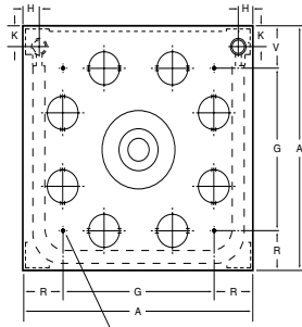
(4) MOUNTING HOLES 3/8" - 16 FOR MODELS 40-77 THREAD TAPS
